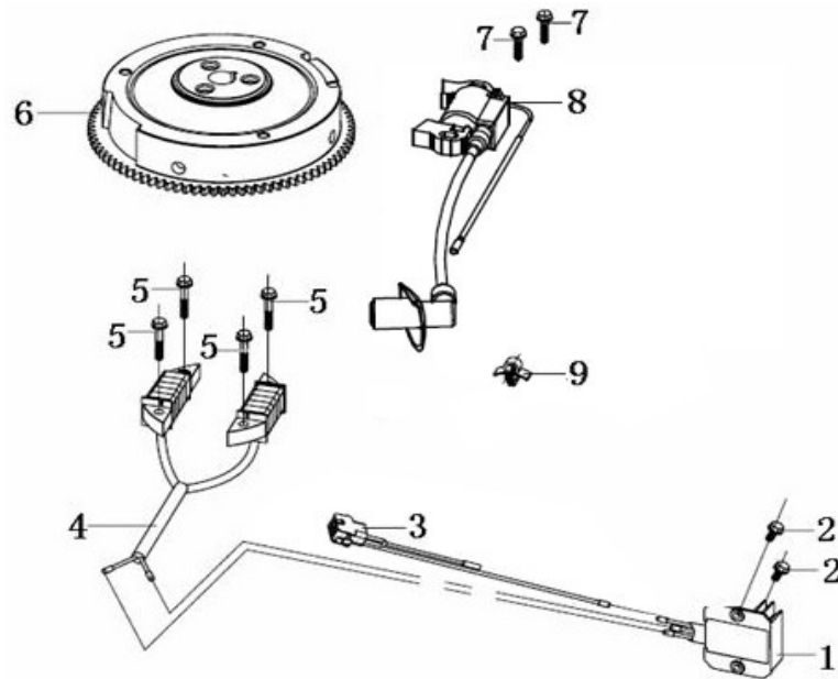
点火系统 (Flywheel1)
